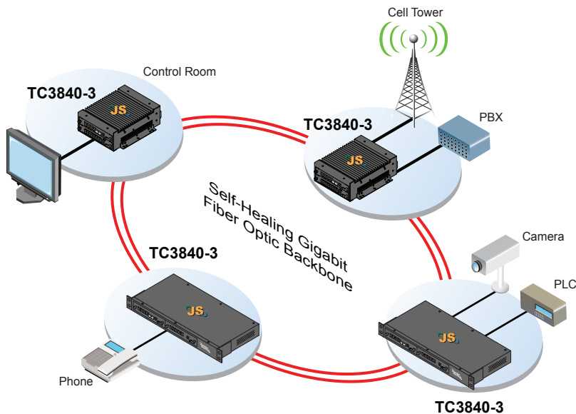
Typical Application Using TC3840-3 Housed in a JumboSwitch 2S & 1U to form a Ring Network
